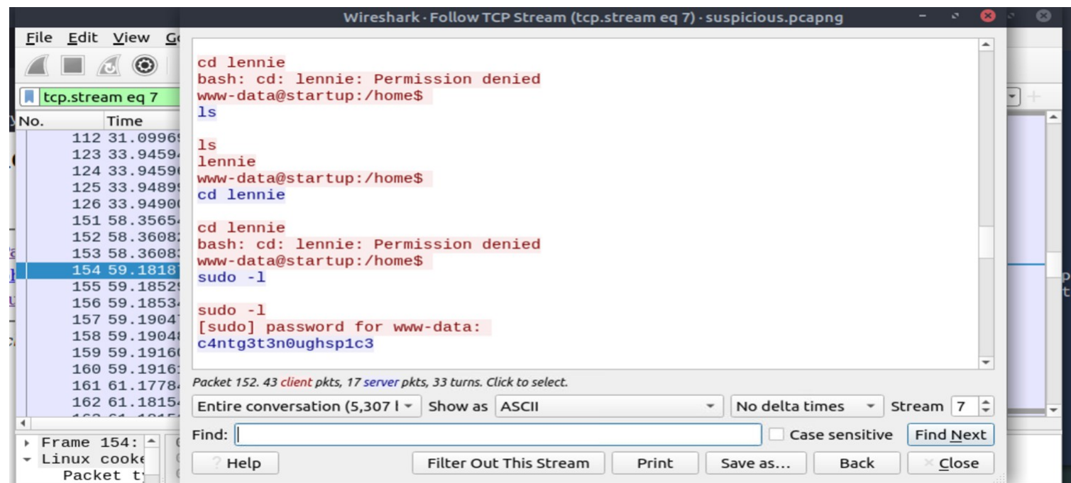
Figure 22: Testing for Local Admin Password Re-Use
